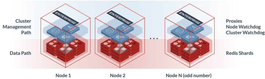
Fig 1: Shared-nothing Cluster Architecture
